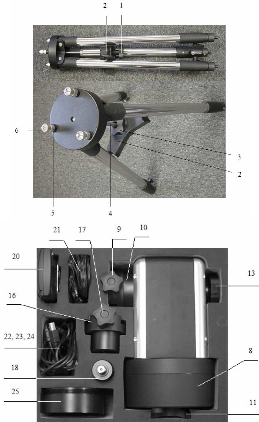
Figure 5. MiniTower packages
